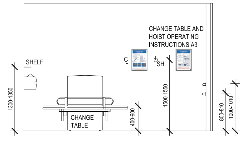
ELEVATION D
