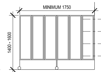
PRIVACY SCREEN
