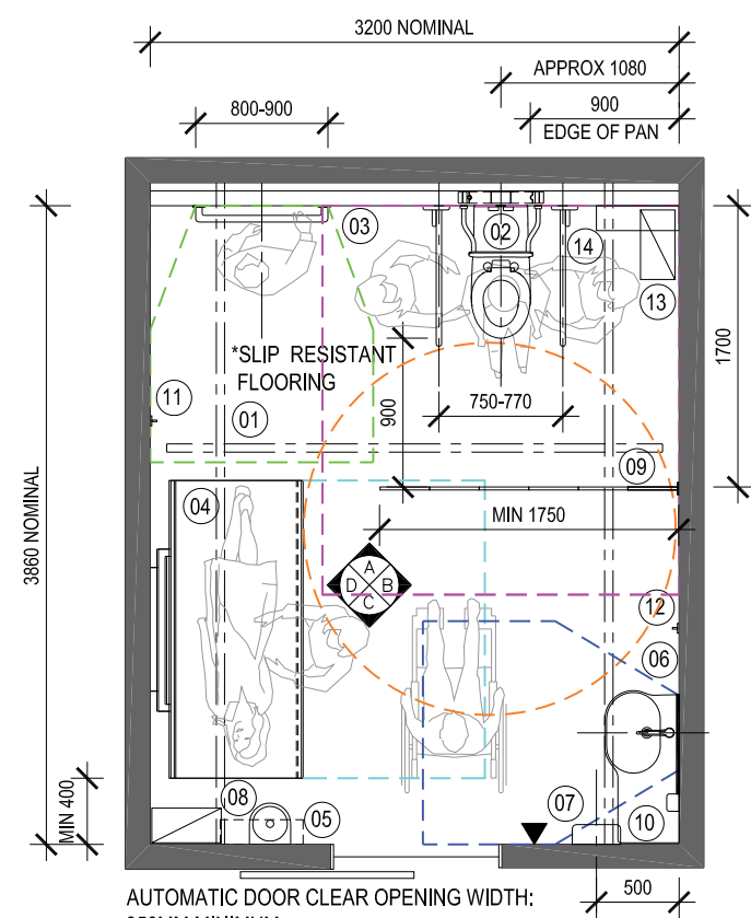
DESIGN 1A WITHOUT SHOWER RECTANGULAR
