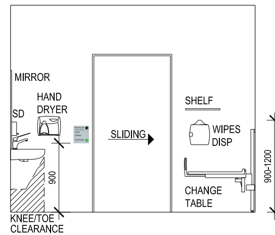
ELEVATION C
