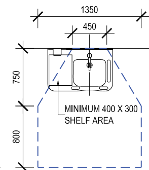
BASIN
